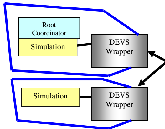
Figure 8: Connecting Two DEVS Domains
