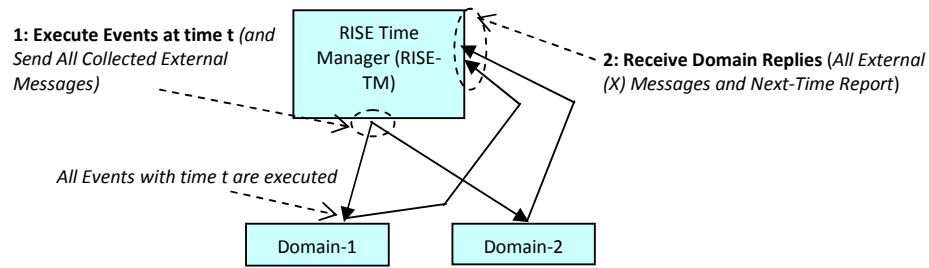
Figure 26: RISE Conservative-based Simulation Cycle at Time t
