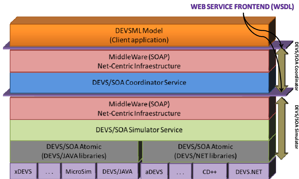
Figure 1. DEVS/SOA architecture
