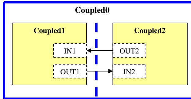
Figure 7: Coupled model partitioned across DEVS Domains
