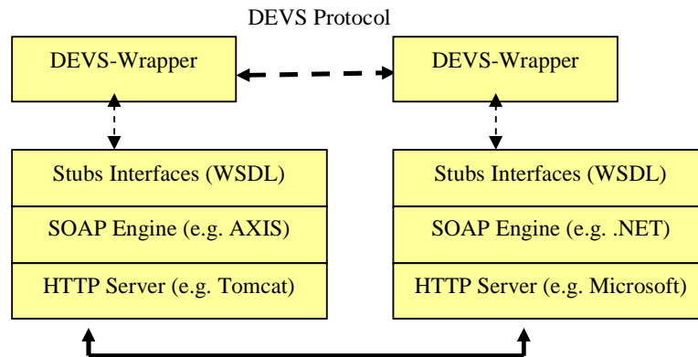
Figure 9: Connecting Domains using Web-Services
