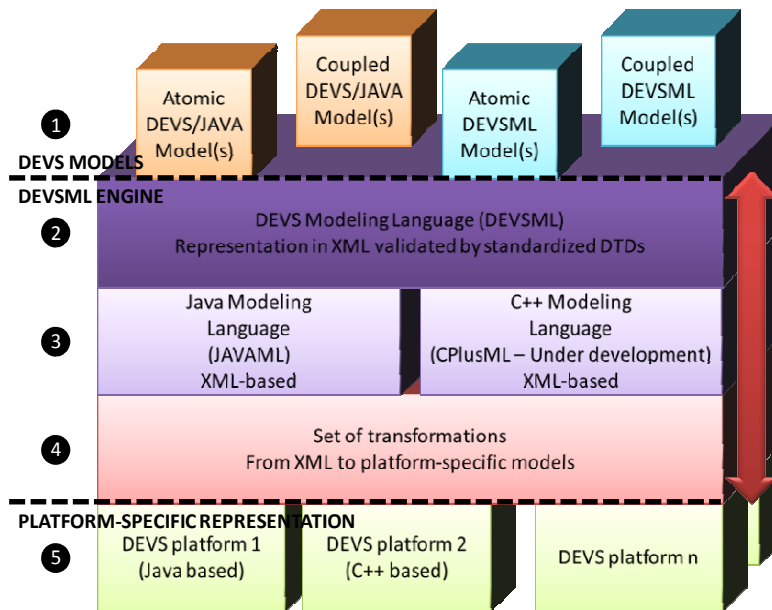
Figure 1: DEVSML layered architecture
