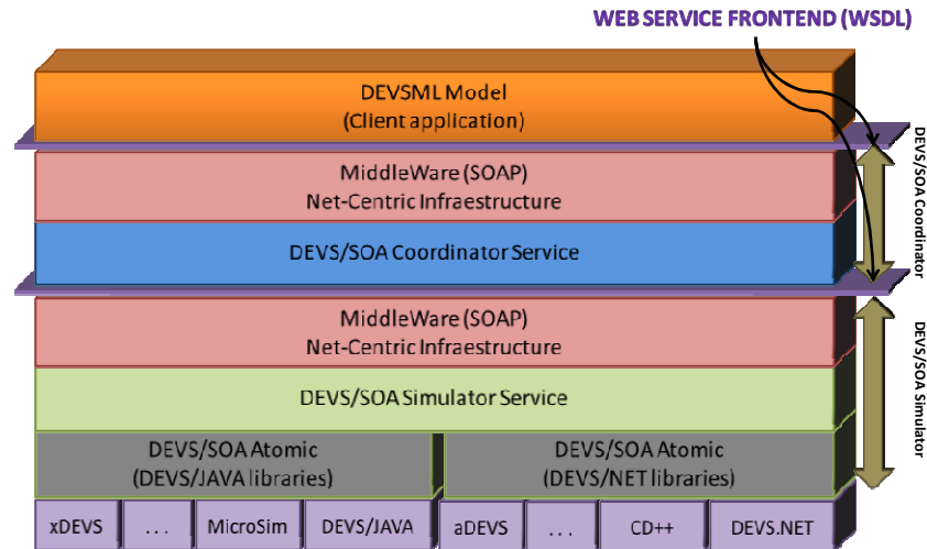
Figure 9. DEVS/SOA architecture
